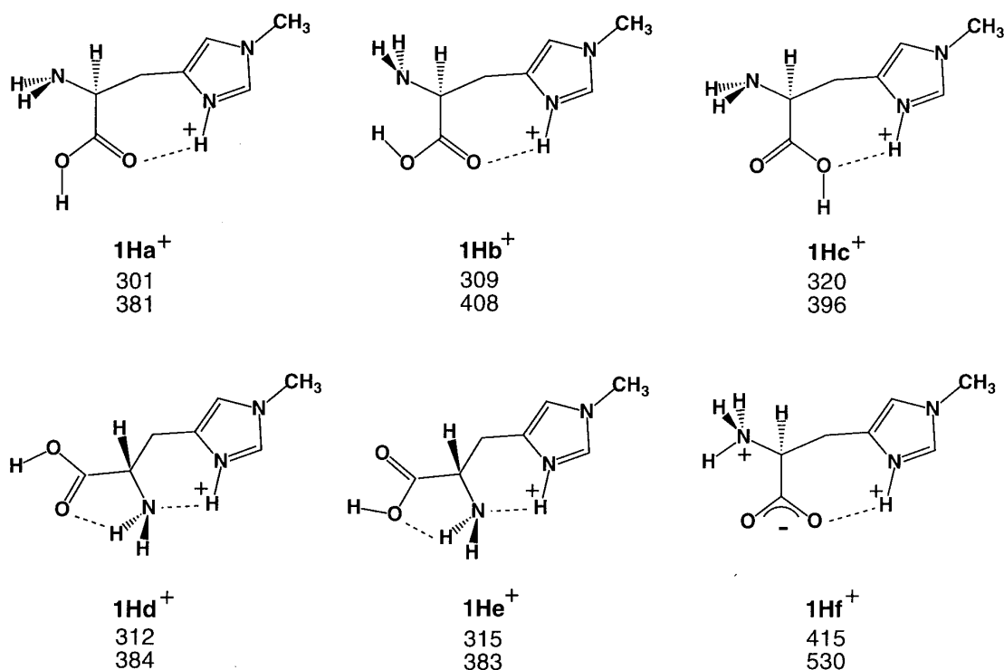
Figure 3. Optimized structures and heats of formation for 1H + isomers. Top values, AM1 enthalpies; bottom values, PM3 enthalpies.
