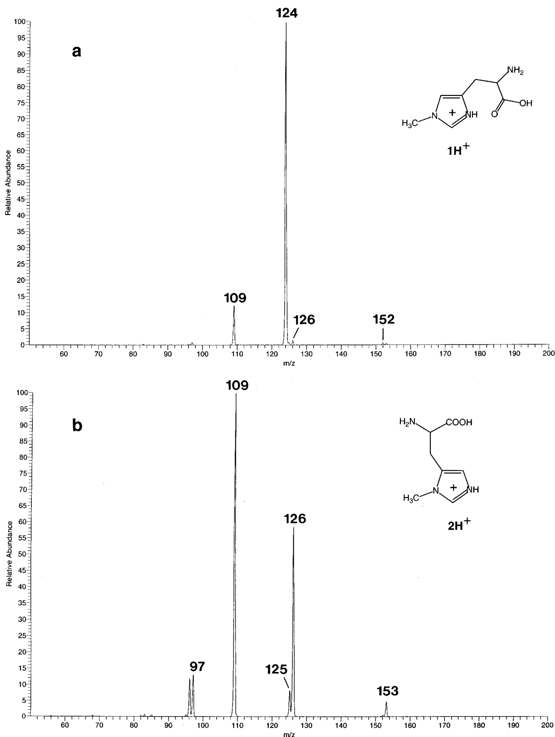
Figure 1. Electrospray ionization ion trap tandem mass spectra of (a) 1H^+ and (b) 2H^+ .
