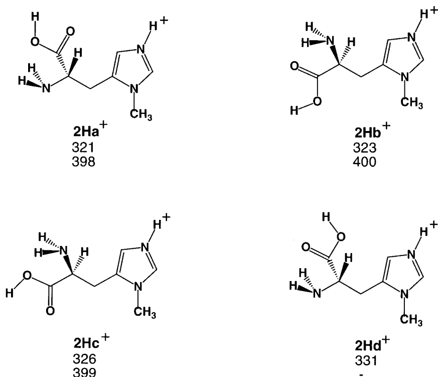
Figure 4. Optimized structures and heats of formation for 2H + isomers. Top values, AM1 enthalpies; bottom values, PM3 enthalpies.
