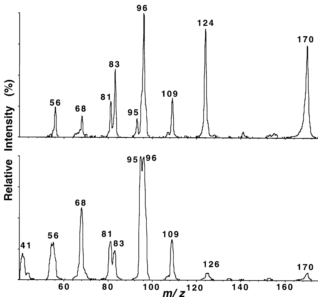
Figure 2. Electrospray ionization tandem quadrupole mass spectra of (top) 1\text{H}^+ and (bottom) 2\text{H}^+ .
